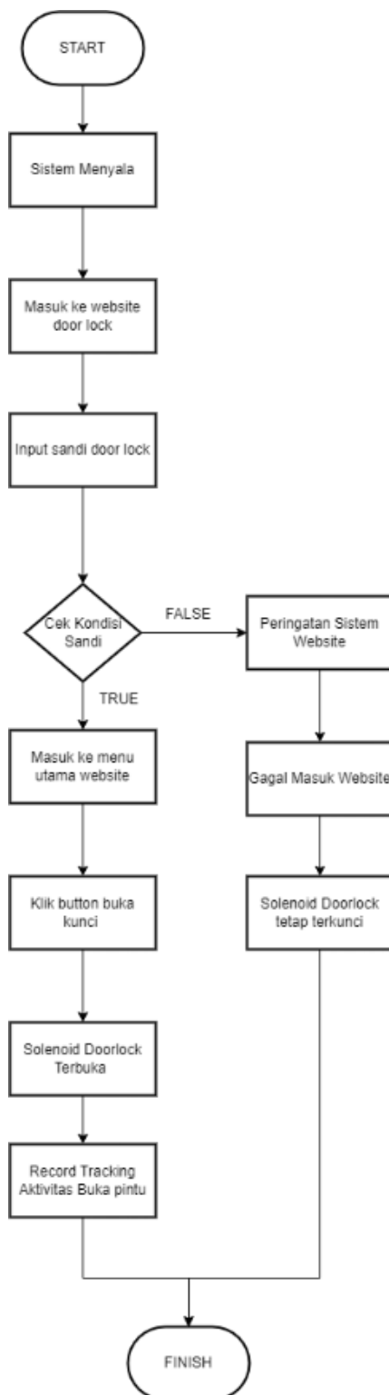
Gambar 2 Flowchart
